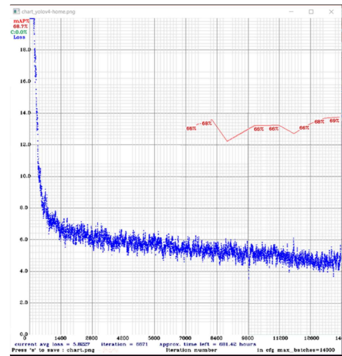
Fig. 23 Model Training
