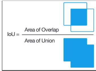
Fig. 25 IoU formula [38]
