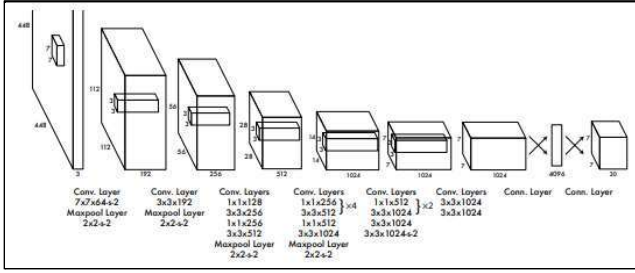
Fig. 10 YOLO architecture [2]
